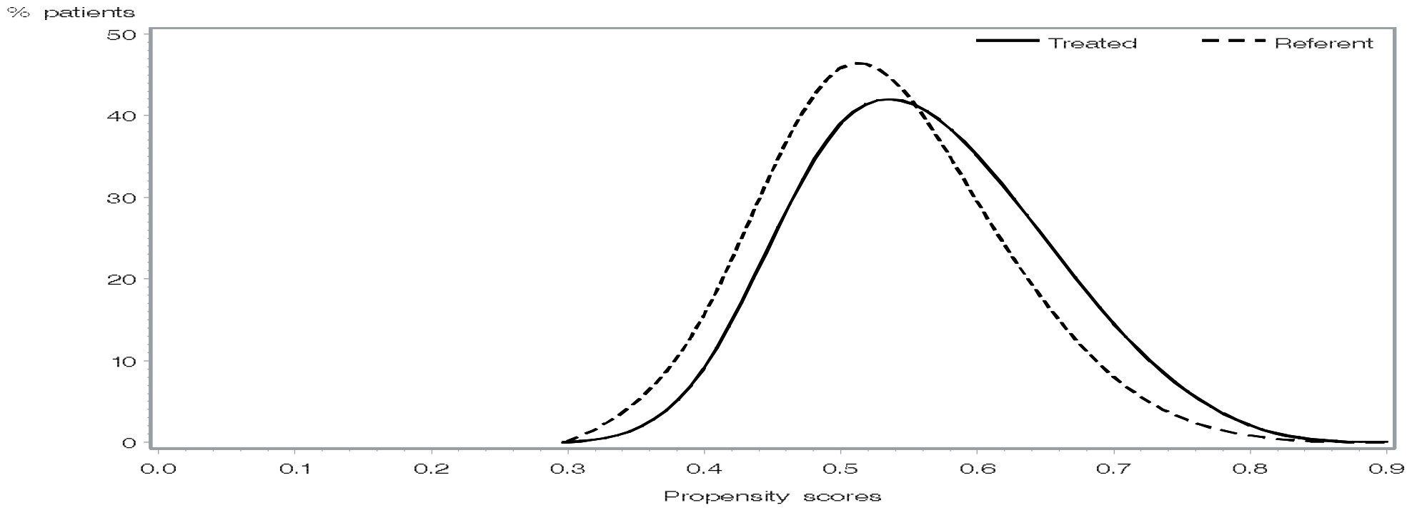
Crude PS distribution
