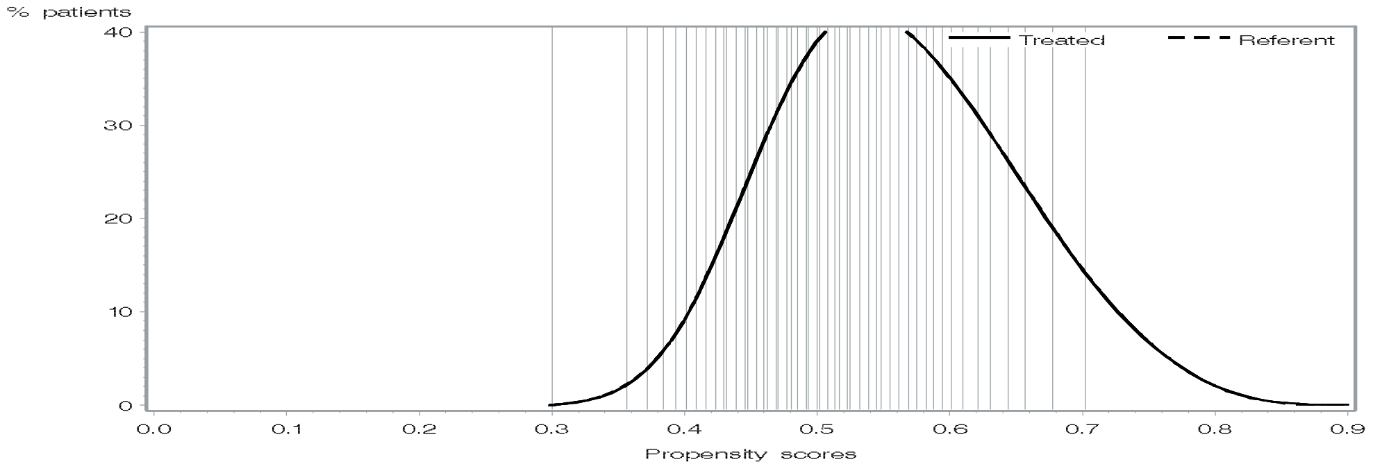
Weighted PS distribution
